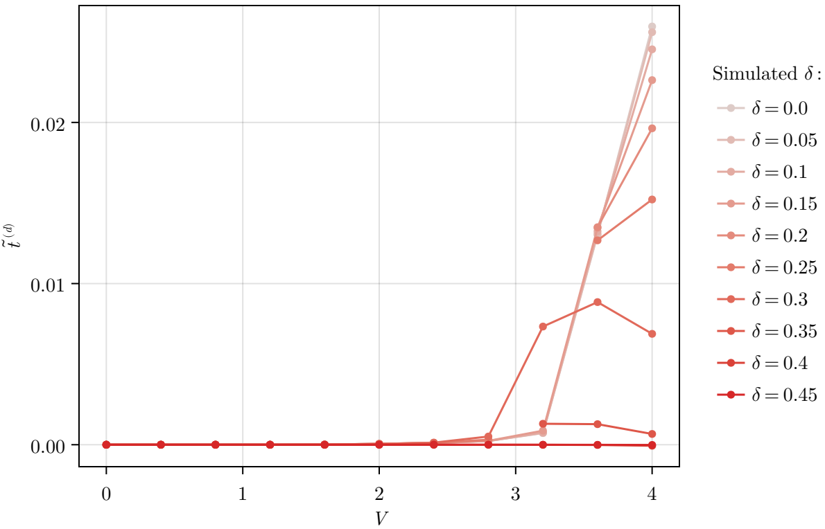
\tilde{t}^{(d)} \ (t=1.0, \ U=5.0, \ L=256, \ \beta=100.0)
